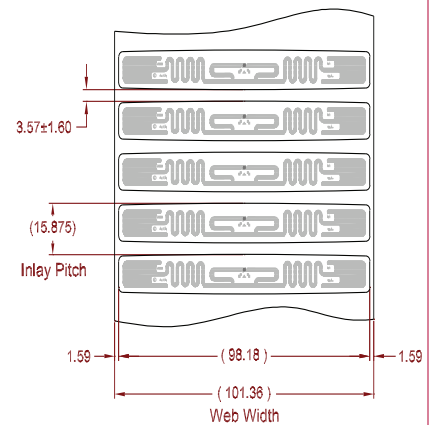
ALN-9640-FWRC / -FWRW (Clear / White Wet Inlay)
